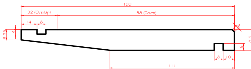
P62 - Western Red Cedar 190 x 18.5mm Standard Bevel Back Weatherboard
