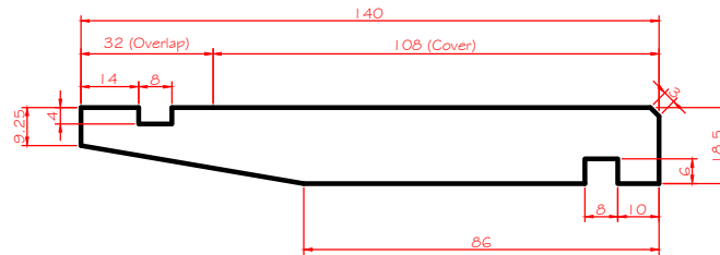
P61 - Western Red Cedar 140 x 18.5mm Standard Bevel Back Weatherboard
