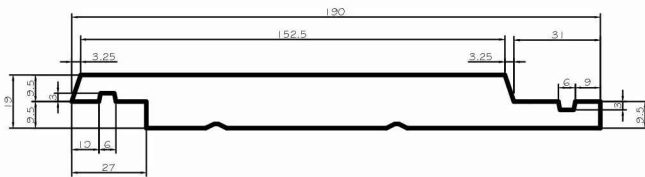
P54: Accoya wood 190 x 19mm Bevelled Centre Grooved Vertical Shiplap Weatherboard
