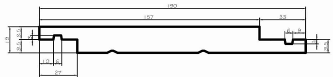
P56: Accoya wood 190 x 19mm Square Vertical Shiplap Weatherboard
