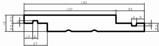
P55: Accoya wood 140 x 19mm Square Vertical Shiplap Weatherboard
